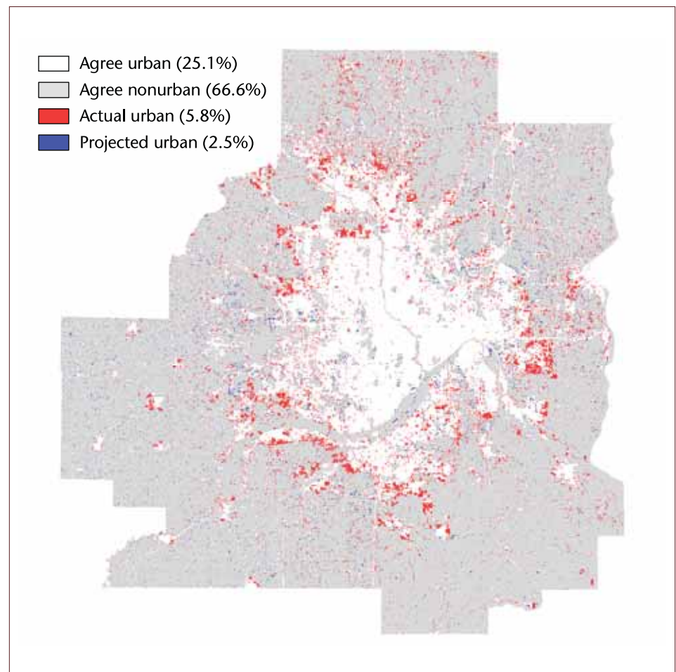
Figure 5. Comparison of Cellular Model of Twin Cities Urbanization with Actual Urbanization from Landsat TM Imagery based on Estimated Quantity of Urbanization, 1986 to 1998
